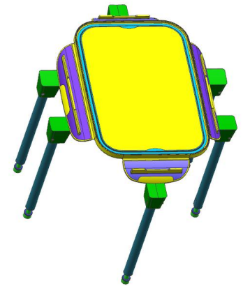
core inserts & ejector block
