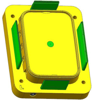
cavity inserts & stripper plate
